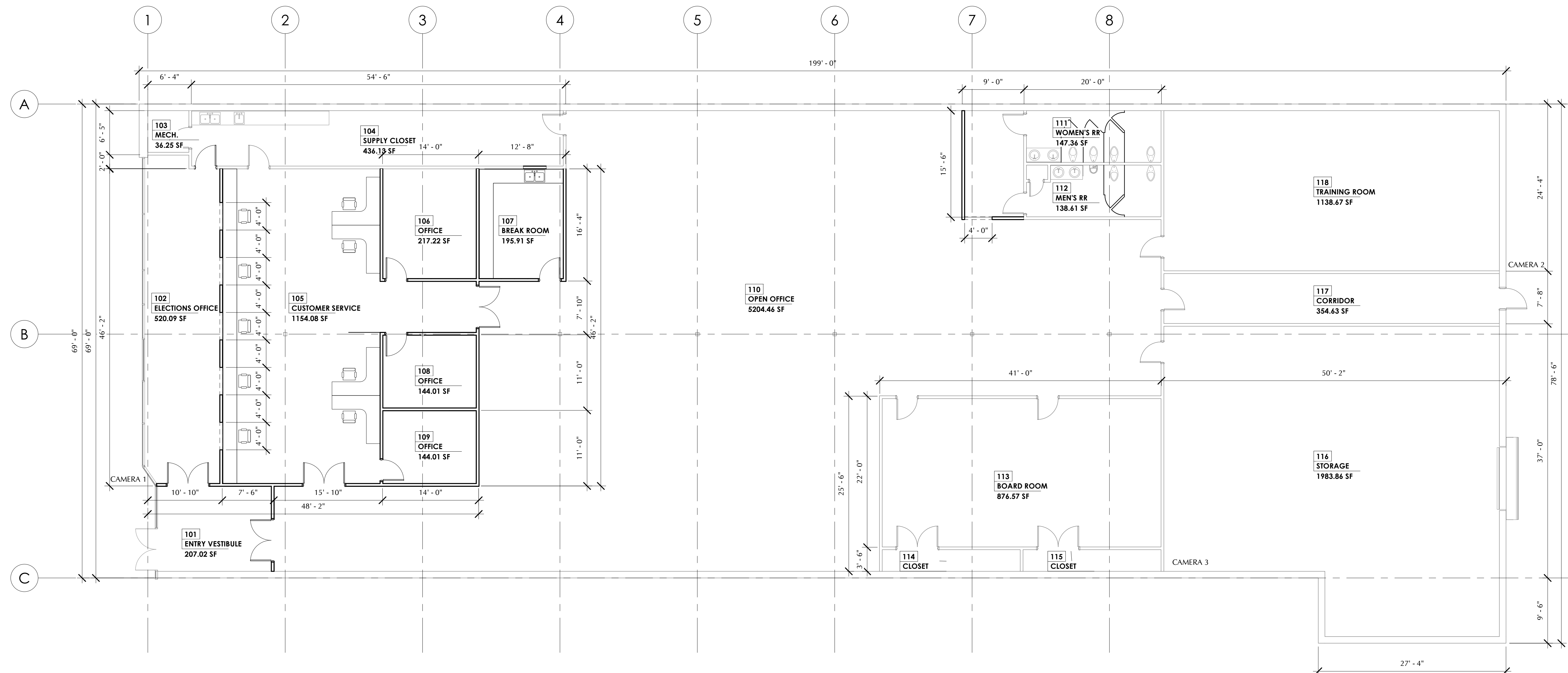
1 FLOOR PLAN A1.1 1/8" = 1'-0"
