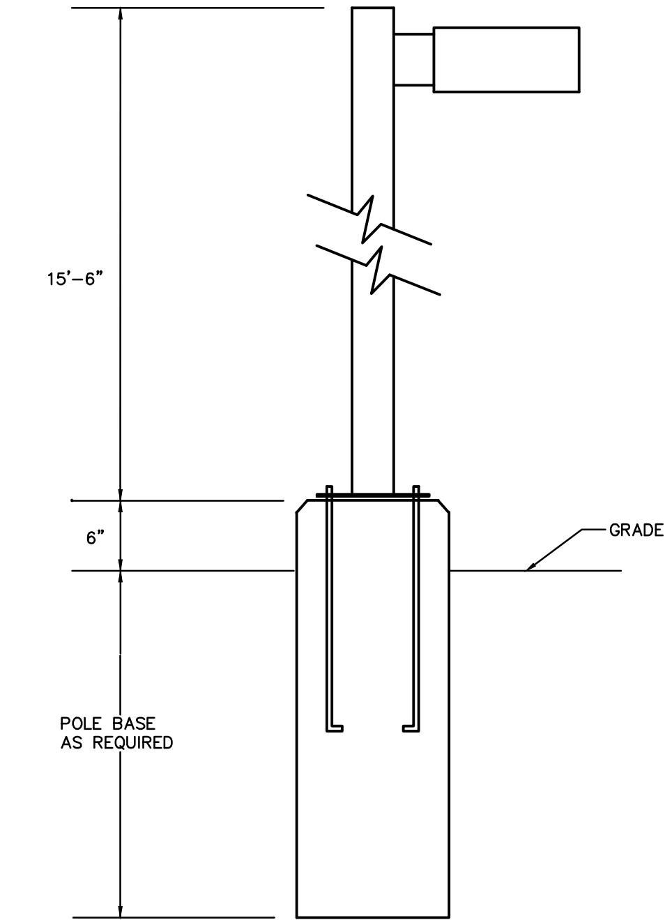
POLE BASE/PARKING LOT LIGHT FIXTURE DETAIL NO SCALE
